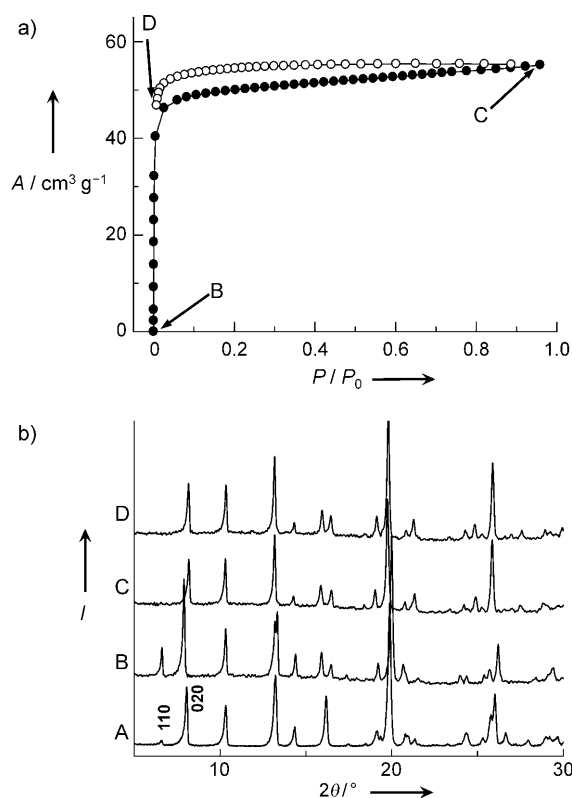
Figure 2. a) CO 2 adsorption (●) and desorption profiles (○) of 1 at 195 K. A: amount adsorbed at STP (standard temperature and pressure). P / P 0 is relative pressure; P 0 of CO 2 at 194.7 K is 101.3 kPa. b) A: XRPD pattern of as-synthesized 1 · x S measured at ambient temperature; B–D: XRPD patterns of 1 measured under CO 2 sorption conditions using CuK \alpha radiation. Each pattern corresponds to the points labeled in (a).
